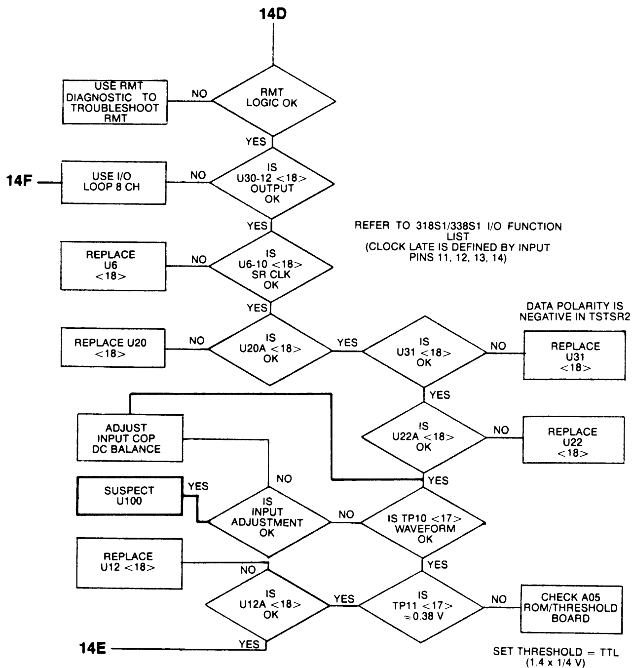
Figure 7-57. Troubleshooting Tree 14: SER A07 TSTSR2 (Sheet 3 of 4).
