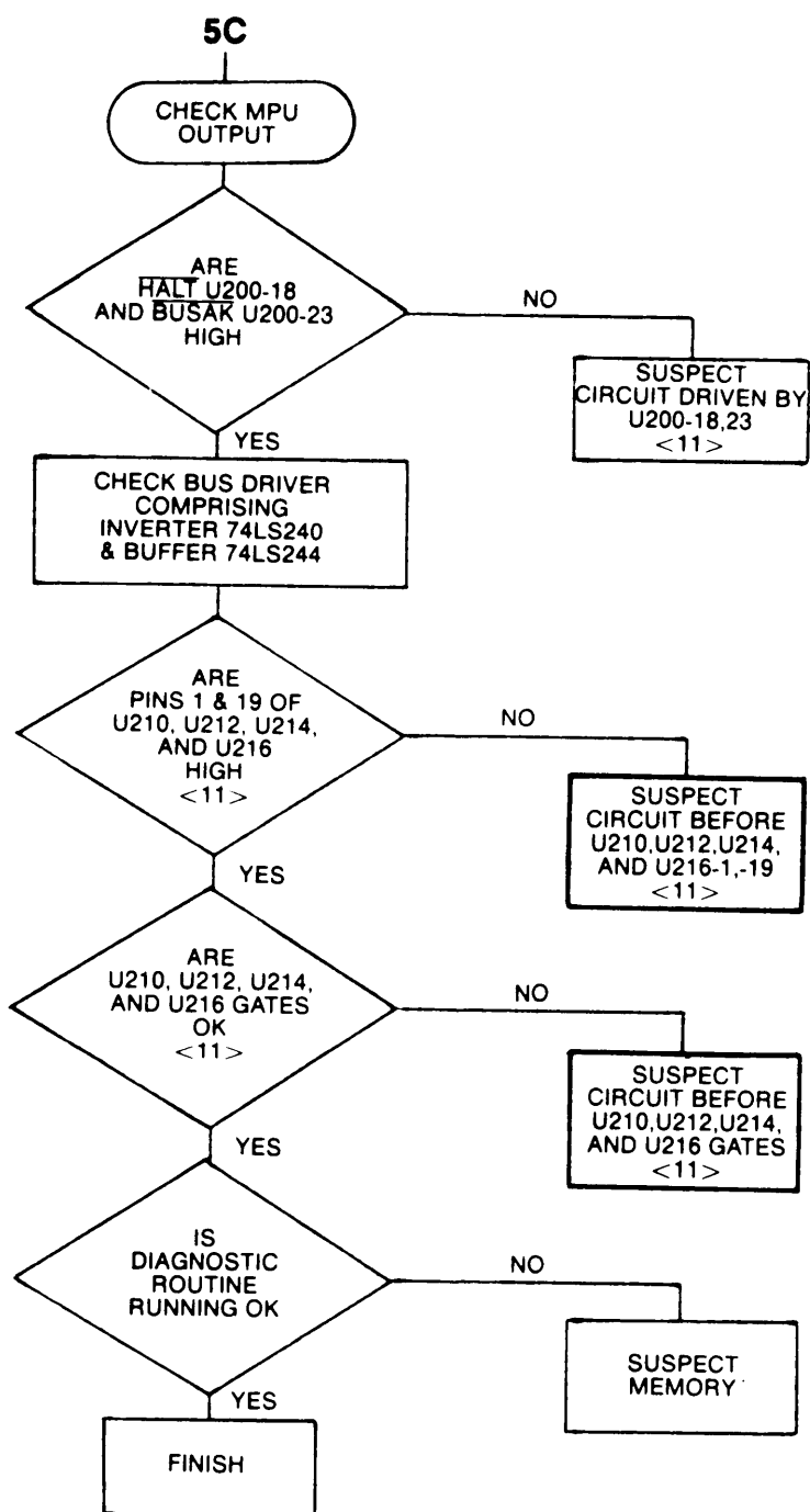
Figure 7-48. Troubleshooting Tree 5: MPU A06 (Sheet 2 of 5).
