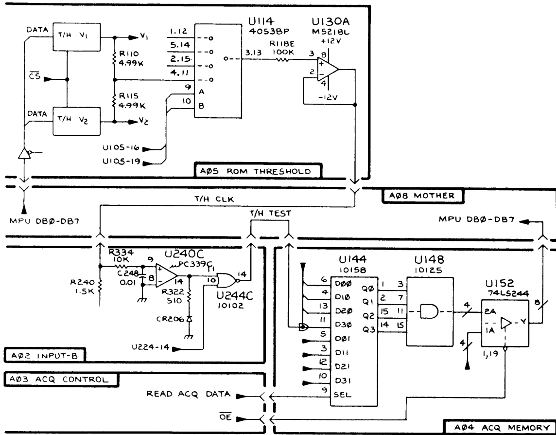
Figure 7-11. 318 Threshold test.
