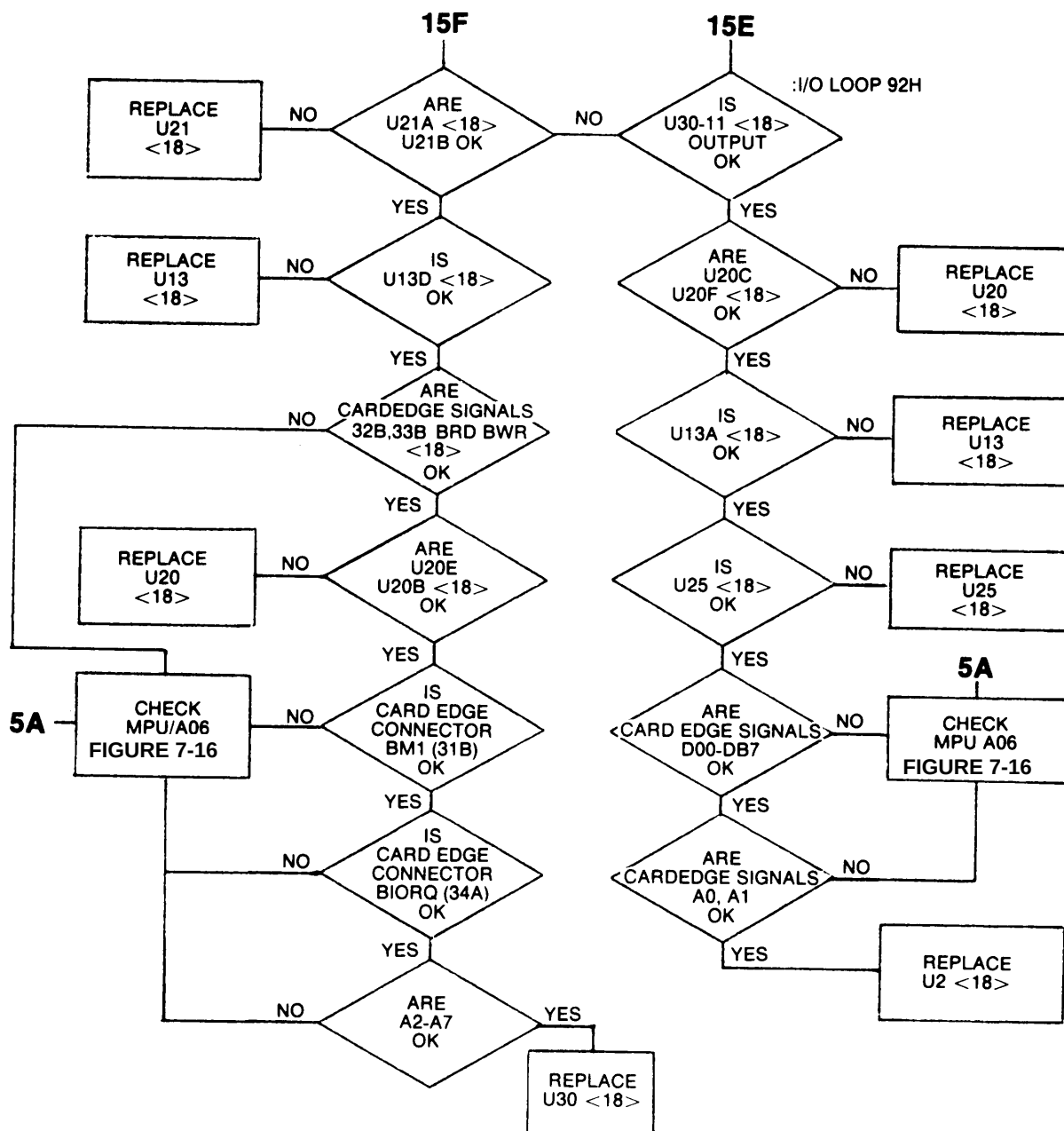
Figure 7-26. Troubleshooting Tree 15: RMT A07 (TSTRM2) (Sheet 4 of 4)
