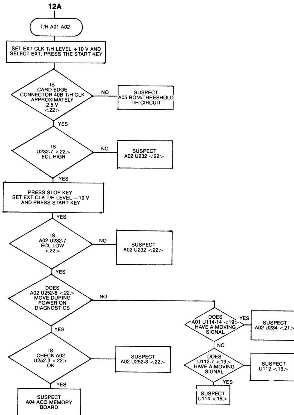
Figure 7-55. Troubleshooting Tree 12: T/H A01 A02
