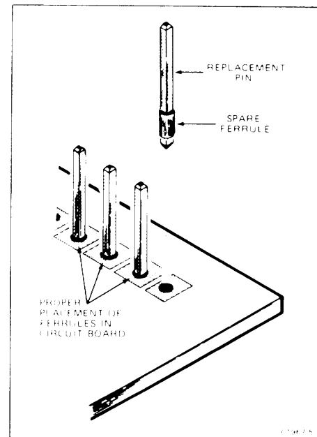
Figure 6-2. Circuit board pin replacement.
