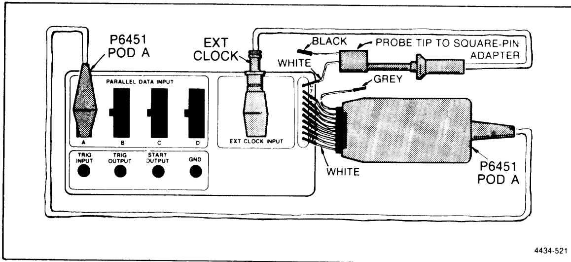
Figure 5-41. 338 Parallel data acquisition check setup.
