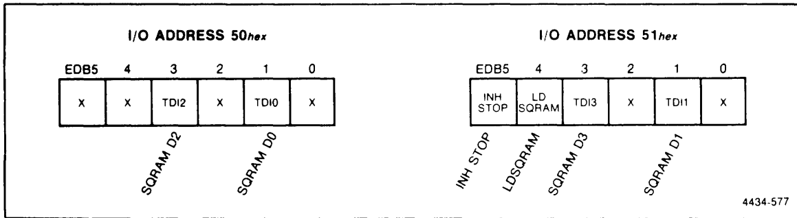
Figure 4-18. 338 SQGRAM data register format.
