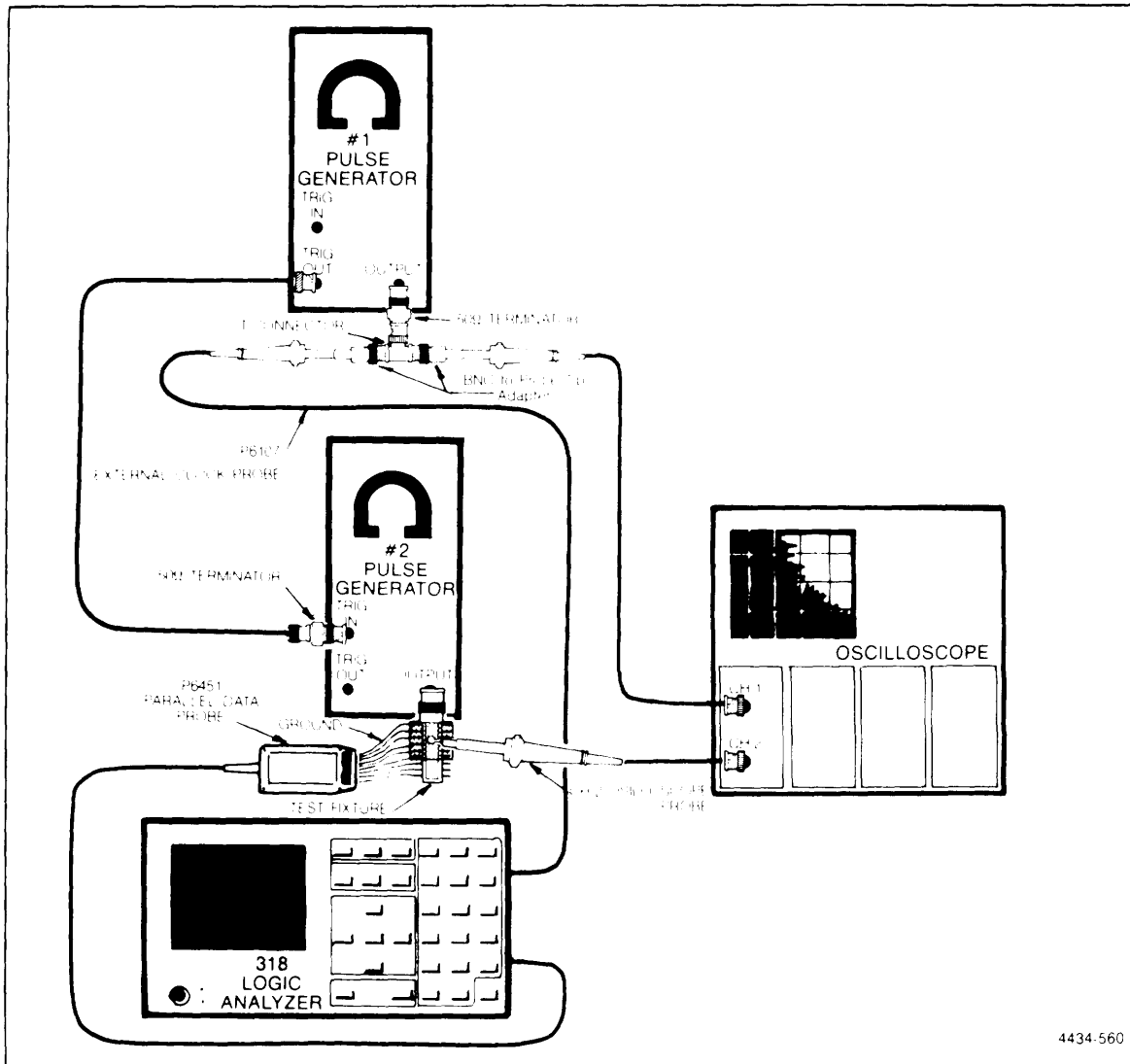
Figure 5-31. 318 Glitch data acquisition test setup.
