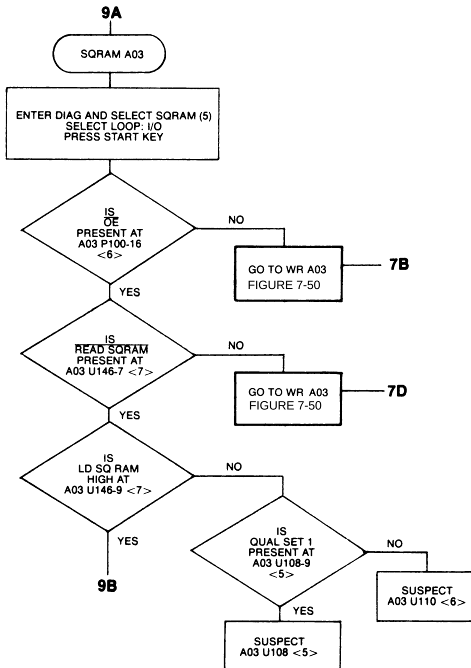
Figure 7-52. Troubleshooting Tree 9: SGRAM A03 (Sheet 1 of 4).
