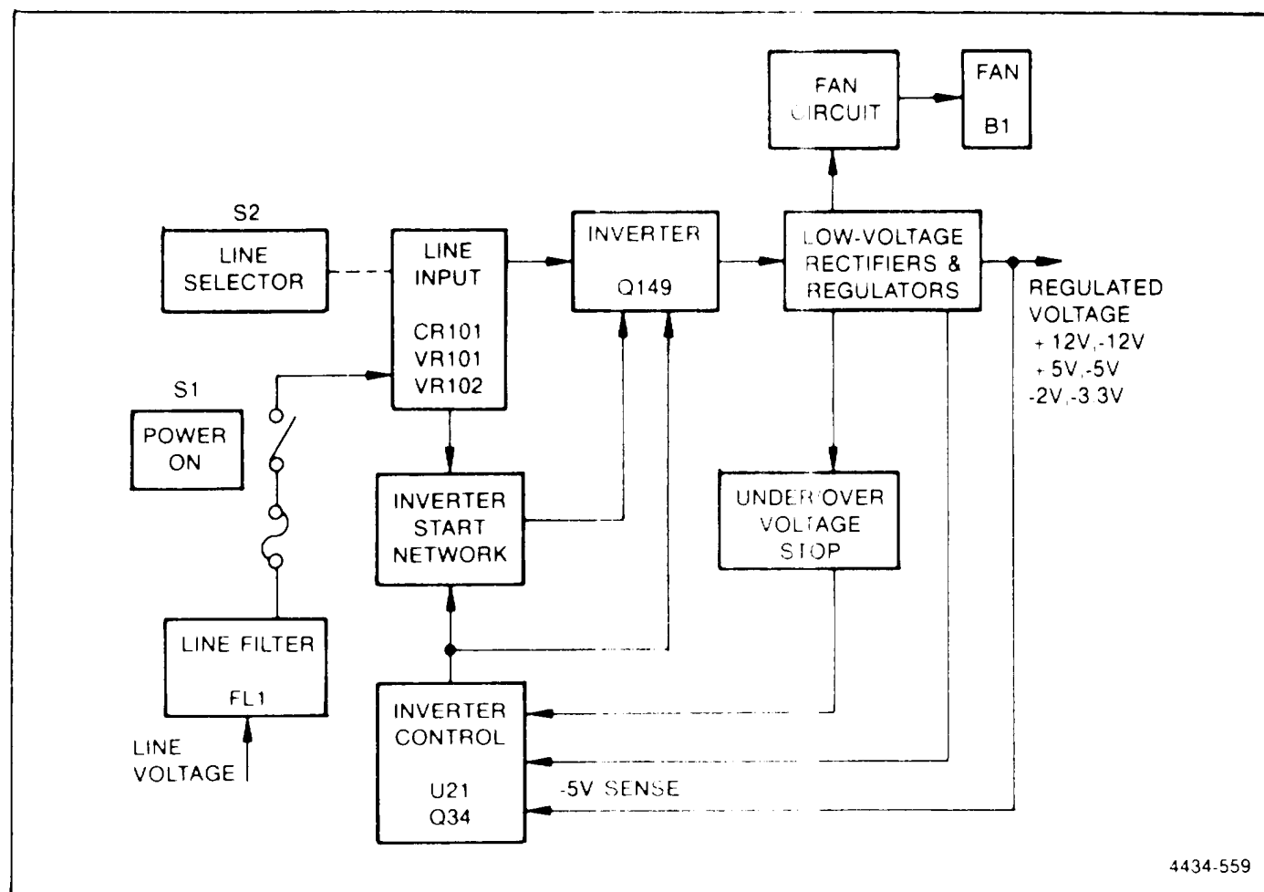
Figure 4-14. 318/338 Simplified diagram of the power supply circuit.
