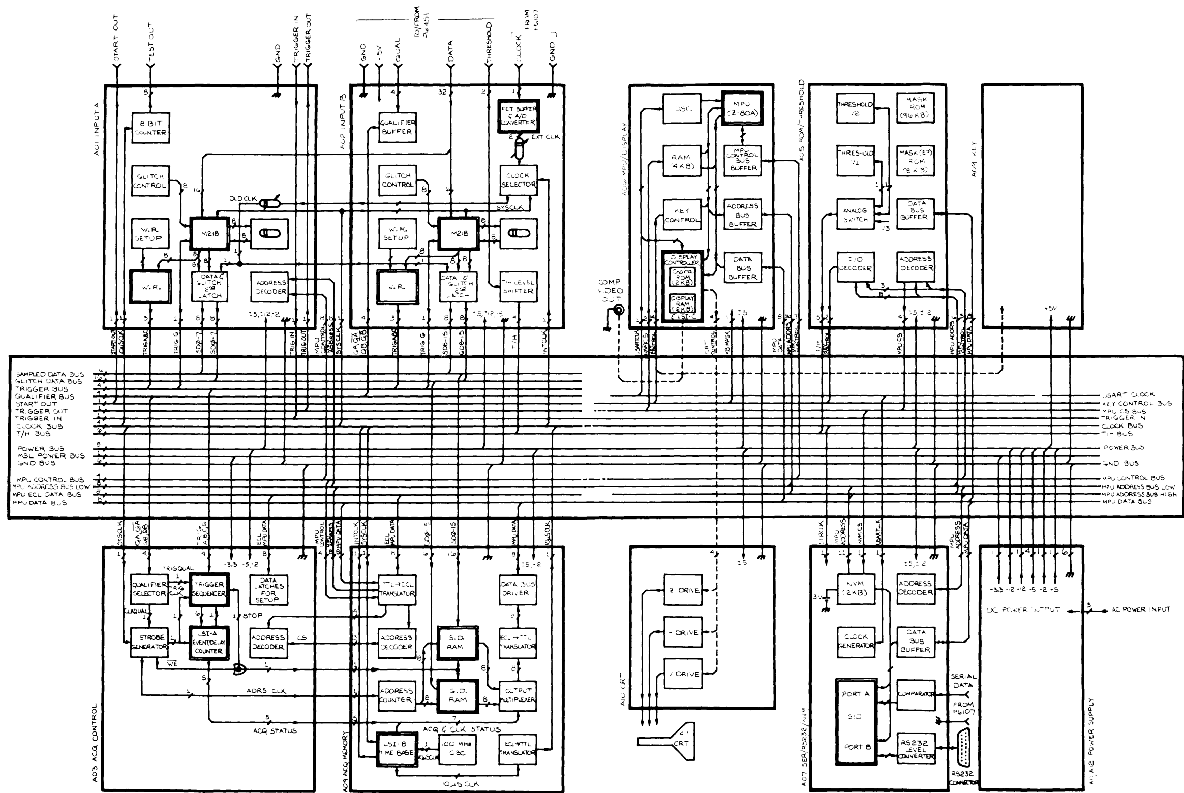
318 Block Diagram
