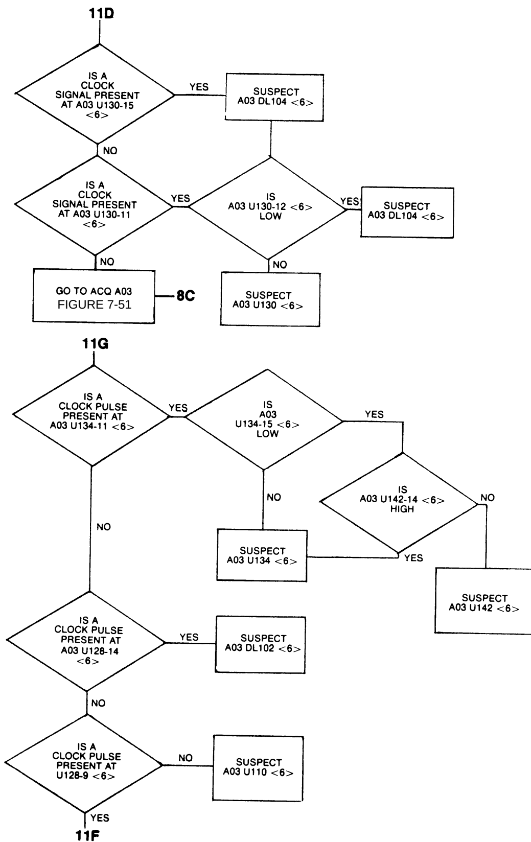
Figure 7-54. Troubleshooting Tree 11: SEQ A03 (Sheet 3 of 4)
