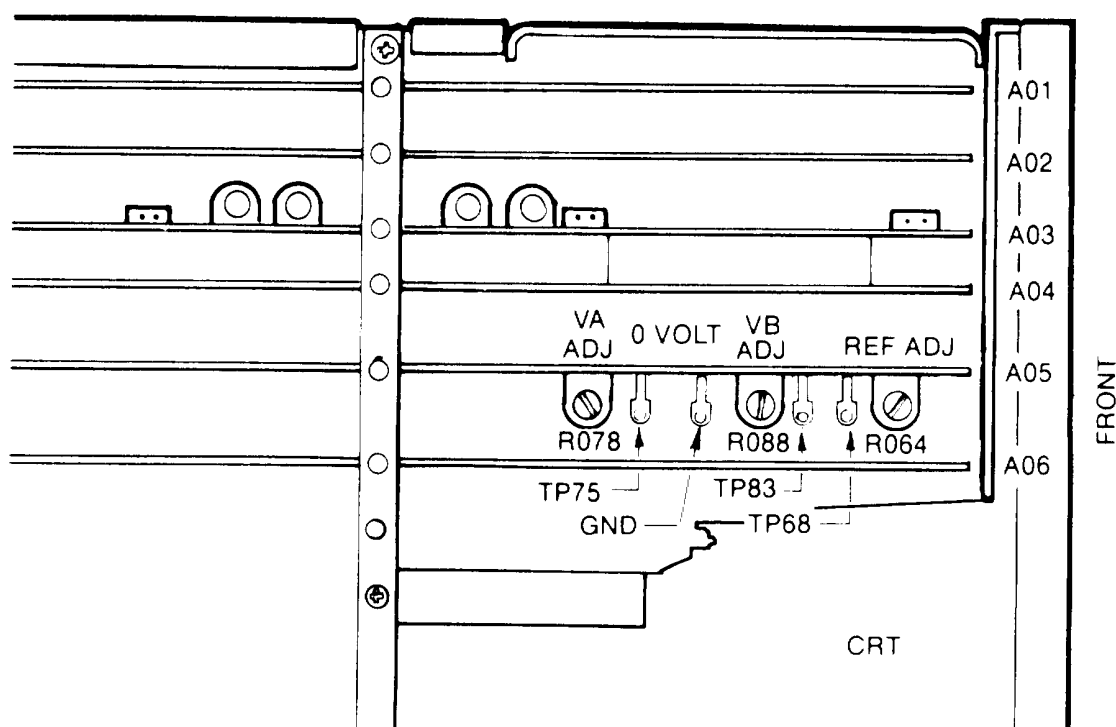
4434-586 Figure 5-16. 318 Threshold voltage adjustments on the the ROM board (A05).
