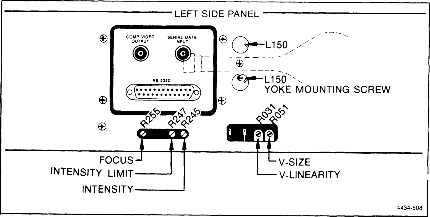
Figure 5-15. 318 CRT adjustments.
