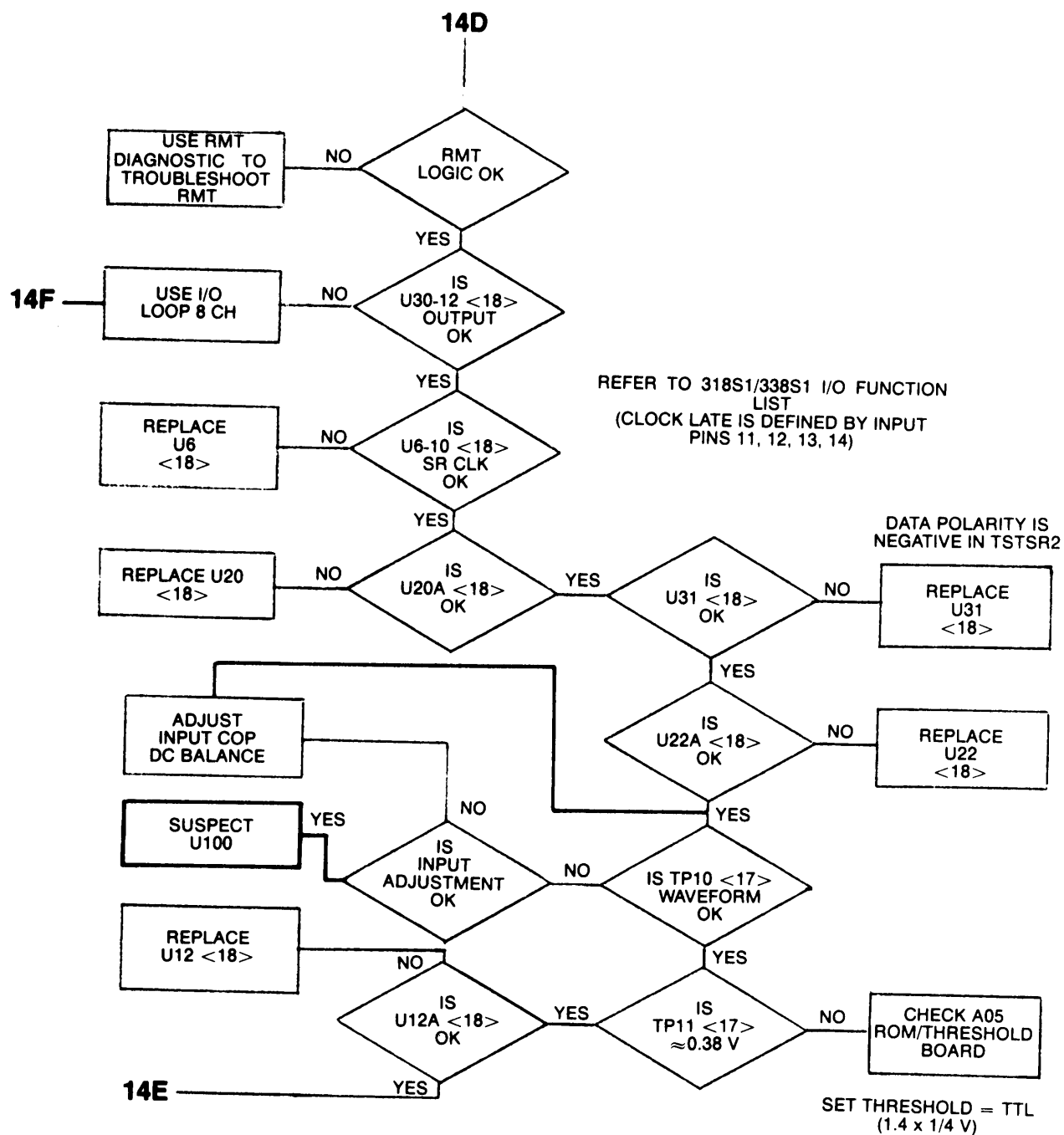
Figure 7-25. Troubleshooting Tree 14: SER A07 (TSTSR2) (Sheet 3 of 4)
