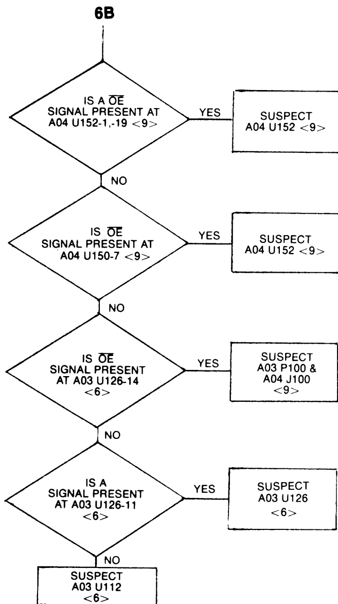
Figure 7-17. Troubleshooting Tree 6. Clock A04 (Sheet 2 of 2)
