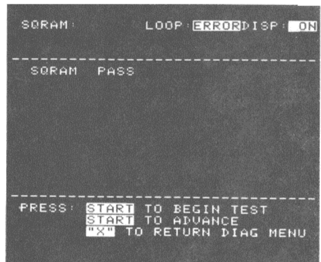
Figure 3-14. Display for trigger sequencer RAM (SQRAM) test.
