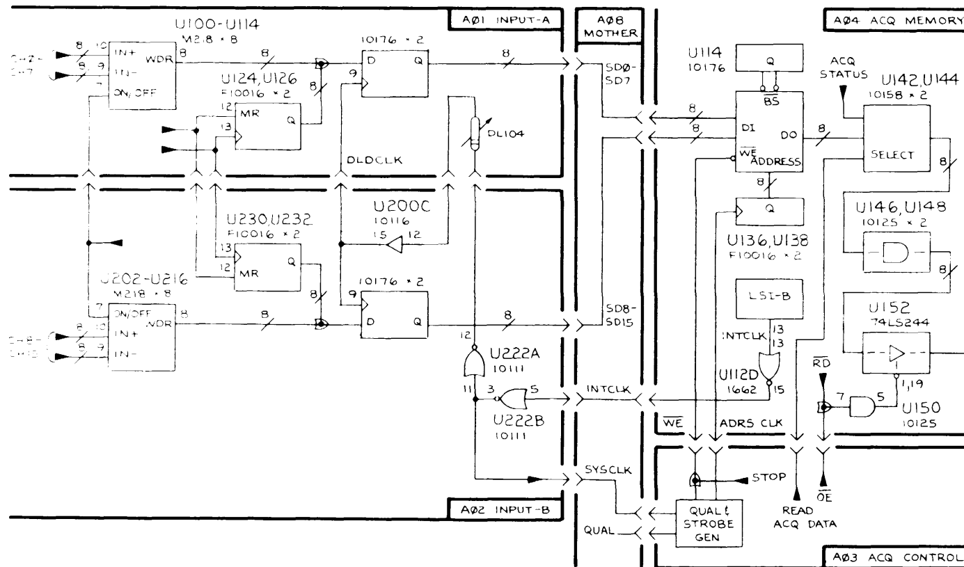
Figure 7-8. 318 ACQ memory test
