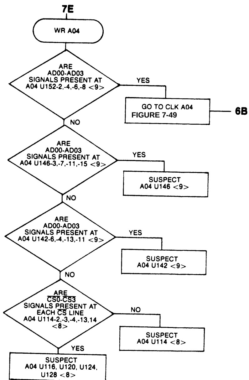
Figure 7-50. Troubleshooting Tree 7: Word Recognizer (WR A01 A02) (Sheet 4 of 4).
