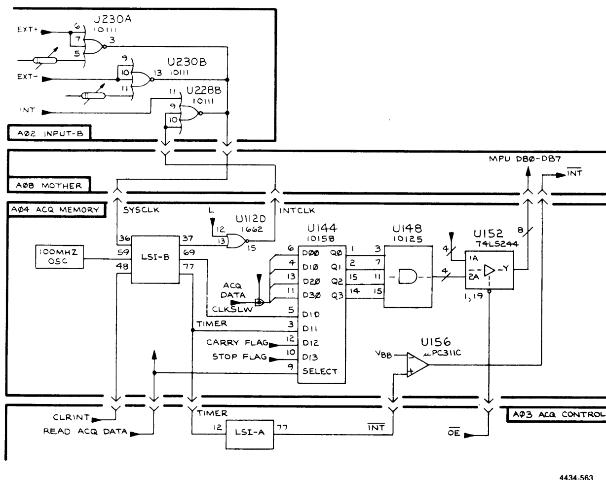
Figure 7-38. 338 Clock test.
