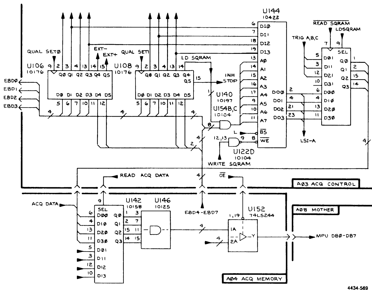
Figure 7-41. 338 SGRAM test.
