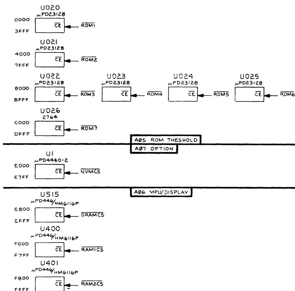
Figure 7-35. 338 Memory map.
