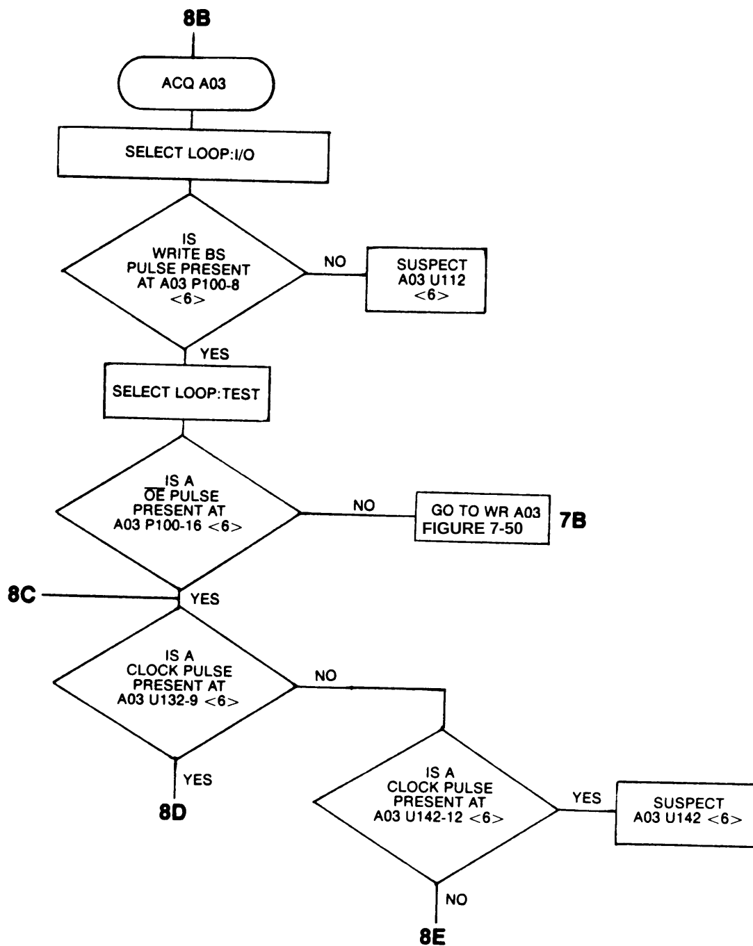
Figure 7-51. Troubleshooting Tree 8: Data Acquisition (ACQ A01 A02) (Sheet 2 of 7).
