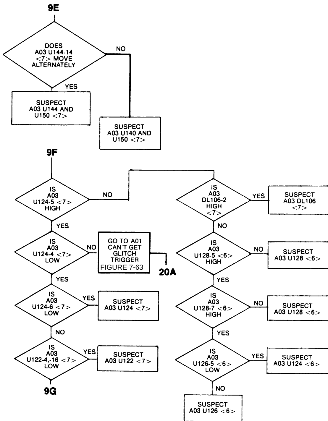
Figure 7-52. Troubleshooting Tree 9: SGRAM A03 (Sheet 3 of 4).
