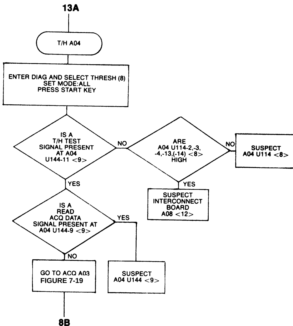
Figure 7-24. Troubleshooting Tree 13: T/H A04
