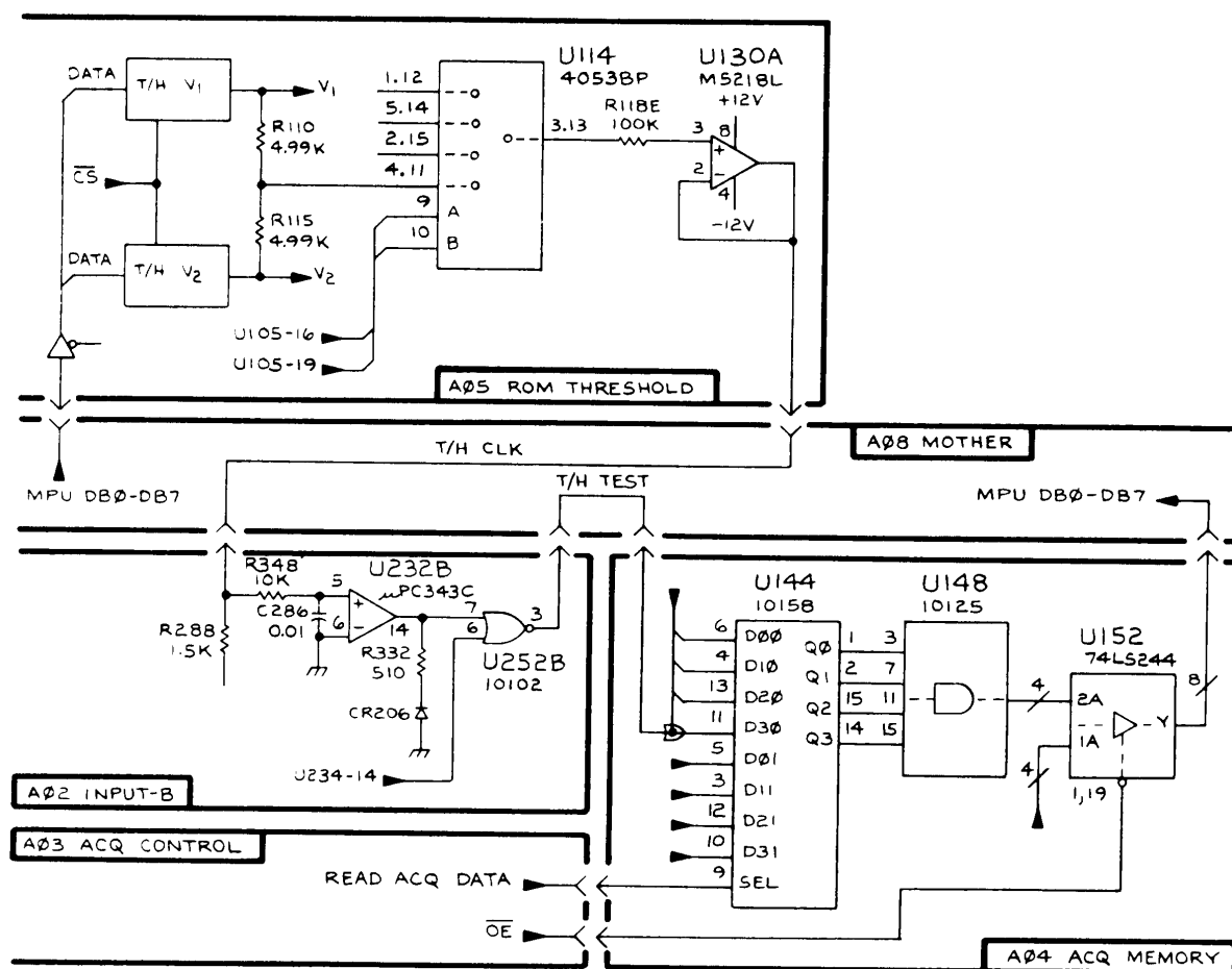
Figure 7-43. 338 Threshold test.
