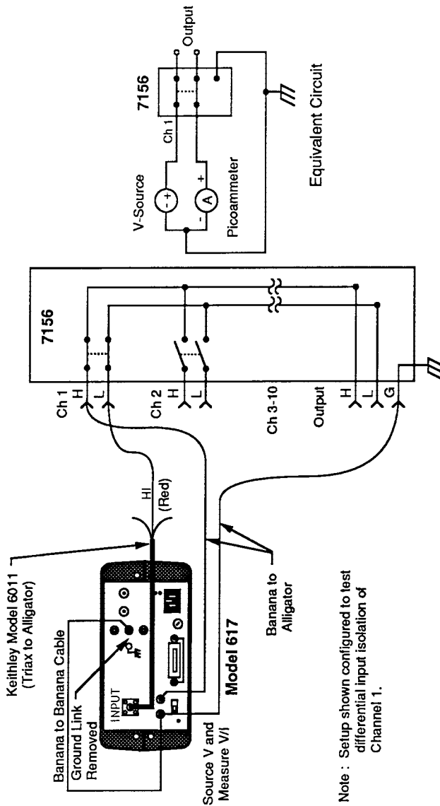
Figure 4-5. Input Isolation (Differential)
