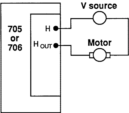
Figure 3-3. Small Motor Control
