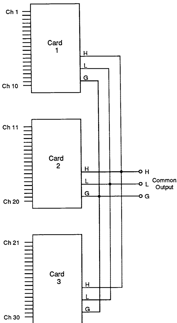
Figure 2-5. Common Output Configuration
