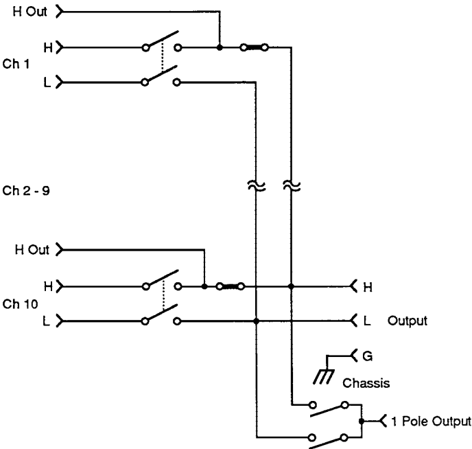
Figure 2-2. Model 7156-M Simplified Schematic
