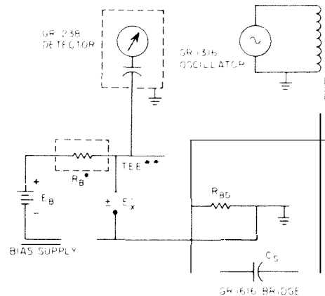
Figure 3-10. Circuit for applying bias to the unknown capacitor - normal configuration. Notes: • Resistor in G874-X Insertion Unit; G874-02 Adaptor provides binding posts for power supply. • G874-T tee with G874-QBJA and G874-QBPA Adaptors to BNC connectors.
