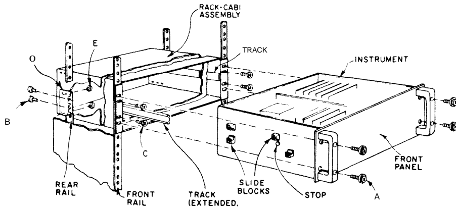
Figure 2-4. Rack-cabinet installation.
