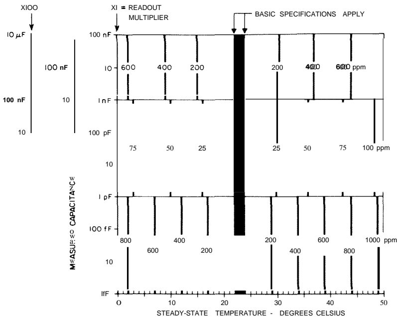
Figure 3-7. Worst-case measurement error due to temperature based on maximum temp coef of C stdsl. Basic specifications apply in shaded band 123°C ±1°C. In remainder of chart the error may add (in the worst case) to the tolerance given in Figure 3-6.
