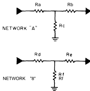
Figure 5-1. Three-terminal conductance standards. R_a = R_b = R_d = R_e = 1 \text{ M}\Omega . R_c = 10.2 \text{ k}\Omega . R_f = 100 \Omega .
