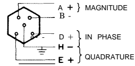
Figure 2-7. DC METER OUTPUTS socket on 1238 Detector, exterior (rear) view.
