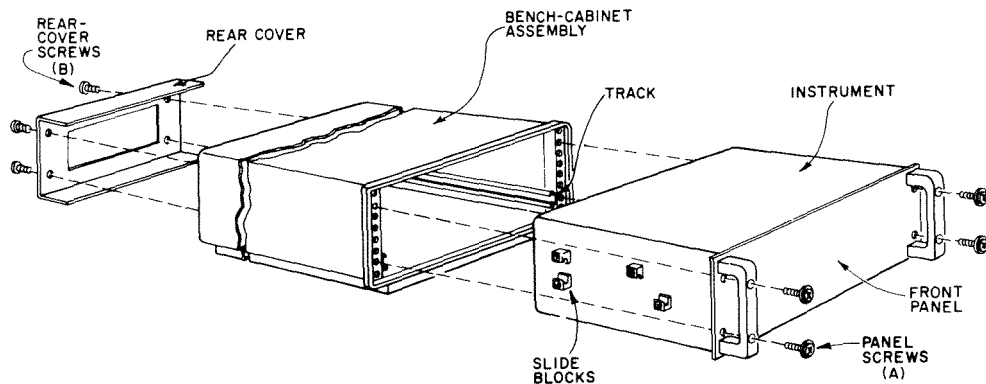
Figure 2-3. Bench-cabinet installation.
