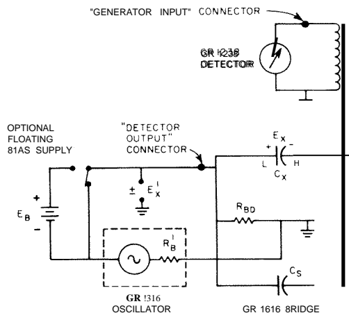
Figure 3-11. Reversed configuration - bridge circuit with oscillator and detector interchanged, showing optional application of bias to unknown capacitor.
