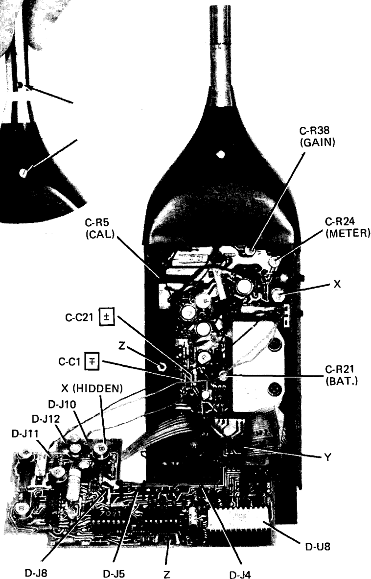
Figure 4-2B. Partial disassembly. The D Board has been swung out, but the instrument will still operate. One screw passes through holes X-X; another, Y-Y; etc. The screw at Z-Z has a small head and requires an insulating washer.
