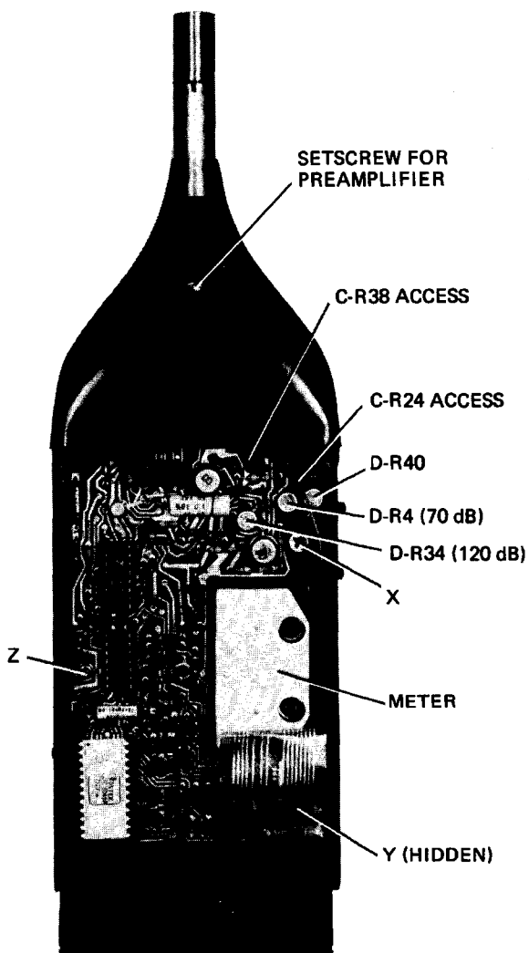
Figure 4-2 A. Rear view with rear cover off.
