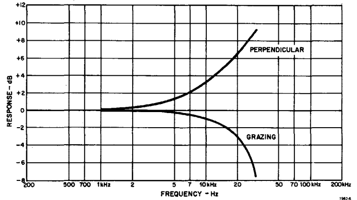
Corrections to be added algebraically to random-incidence response level to find perpendicular- and grazing-incidence free-field response levels.
