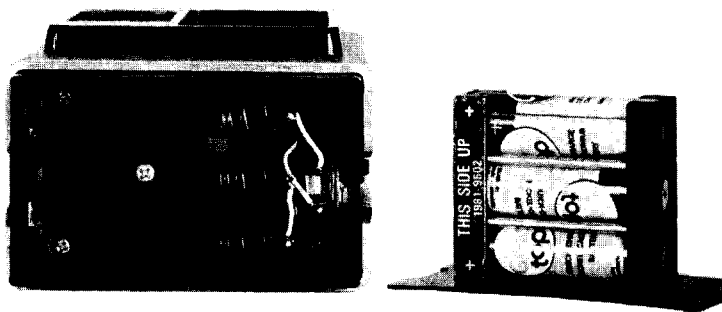
Figure 4-1. Bottom view, with battery-compartment cover and battery pack removed. The 4 screws nearest the corners hold the front and rear panels. Note orientation: middle cell —+, others +-.
