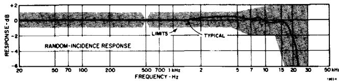
Typical frequency response to random-incidence sound. (Acceptable in gray area.)
