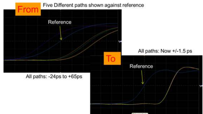
Skews between switch paths are easily maintained with Agilent's unique software
