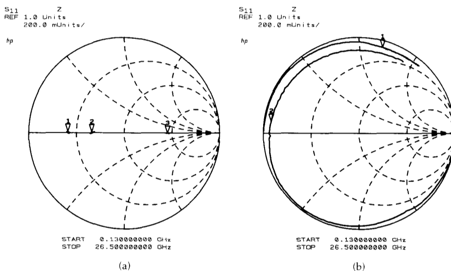
Figure 5 (a) Impedance measurement of 10 ohm (#1), 25 ohm (#2), and 125 ohm (#3) resistors. (b) Impedance measurement of .5 nH inductor (#1) and interdigitated capacitor (#2).
