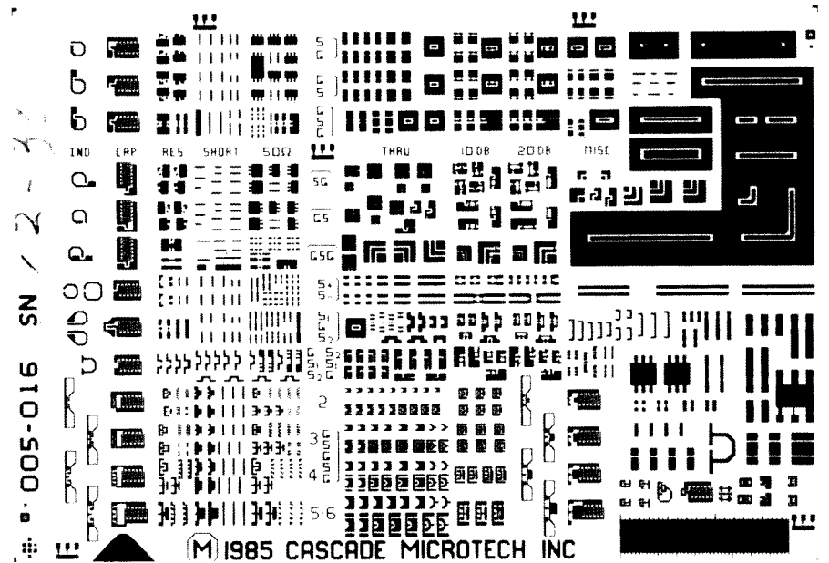
Figure 11 Enlarged view of the Impedance Standard Substrate (ISS). The on-wafer devices shown are used to calibrate at the probe head to wafer interface.
