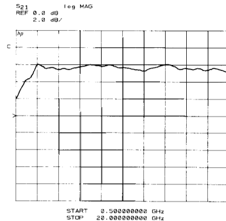
Figure 10 Voltage gain measurement of an on-wafer single stage amplifier MMIC from .5 to 20.0 GHz.
