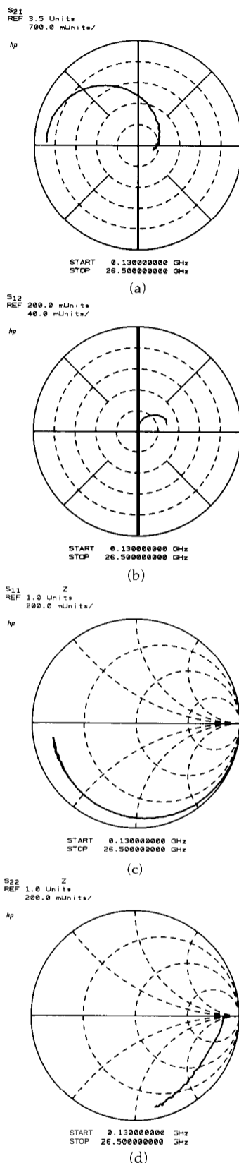
Figure 9 S-parameter measurement of a 1 \times 300 \mu\text{m} GaAs FET using Cascade Microtech probes, (a) S_{21} (b) S_{12} (c) S_{11} (d) S_{22} .
