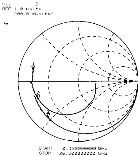
Figure 6 Impedance measurement of the gate-source diode of a GaAs FET, with open drain, at 3 different DC bias conditions: V_{gs} = 1.0 V (#1), V_{gs} = 0.6 V (#2), V_{gs} = 0.0 V (#3).
