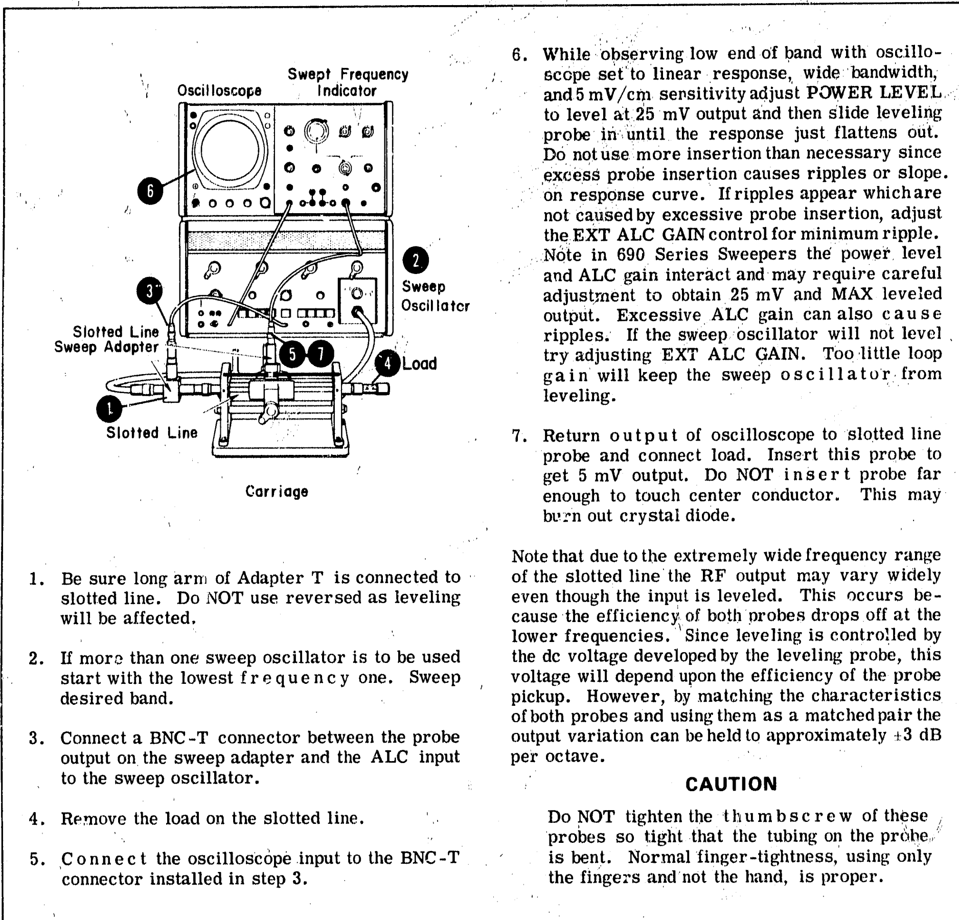
Figure 9. Leveling
