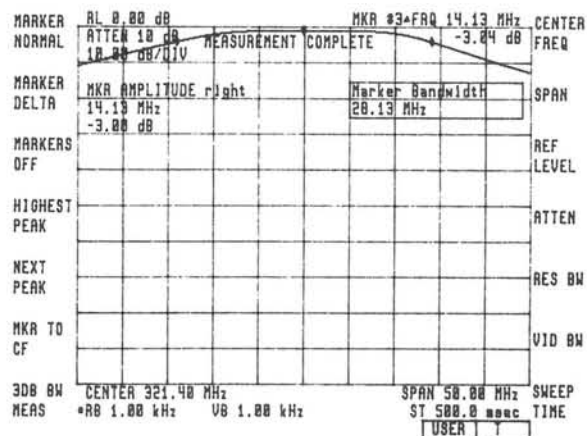
Figure 1-73. 3 dB Bandwidth with 43DB BW MEAS Softkey
