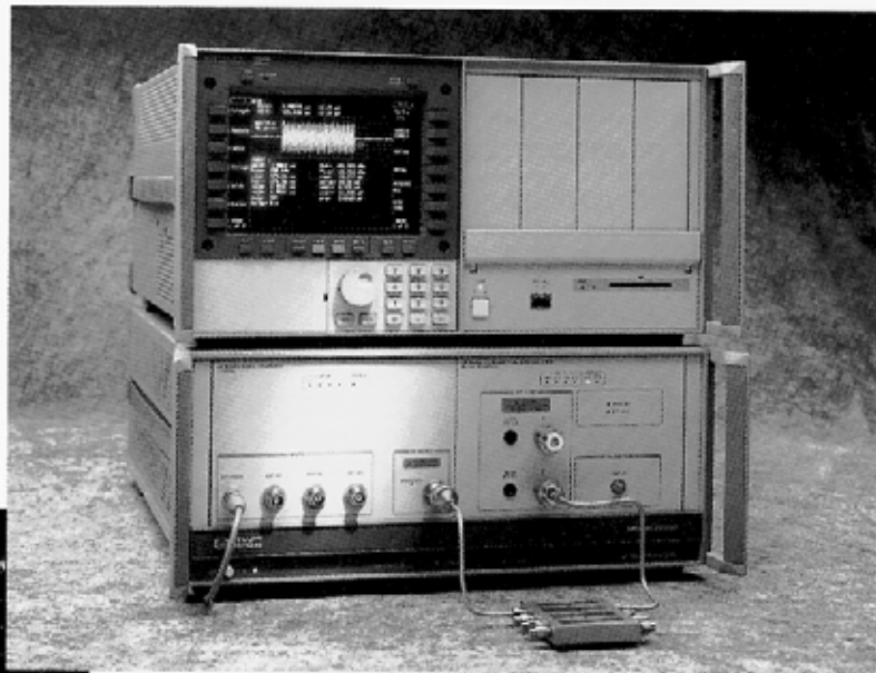
Excellent pulse fidelity makes the HP 70340A an ideal pulsed component and EW receiver stimulus.
