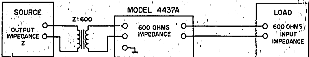
Figure 3-7. Input Matching with Transformer
