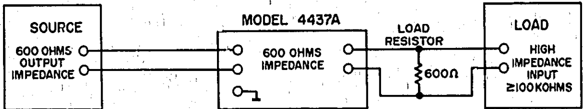
Figure 3-11. Output Matching with Shunt Resistor
