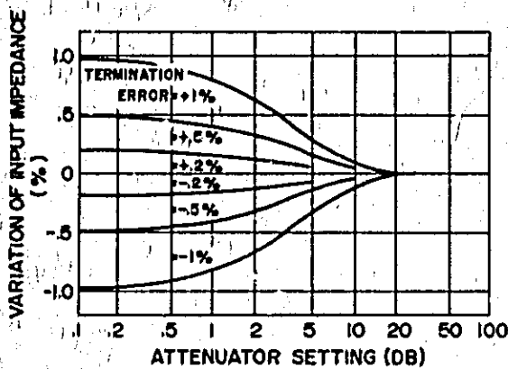
Figure 3-4. Input Impedance Change Due to Terminated Resistance Error
