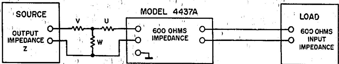
Figure 3-8. Input Matching with Resistive Network
