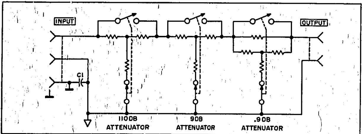
Figure 4-1. Model 4437A Simplified Circuit
