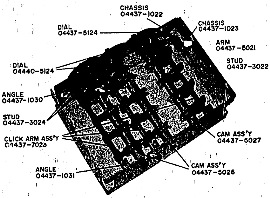
Figure 8-2. Cam Assembly
