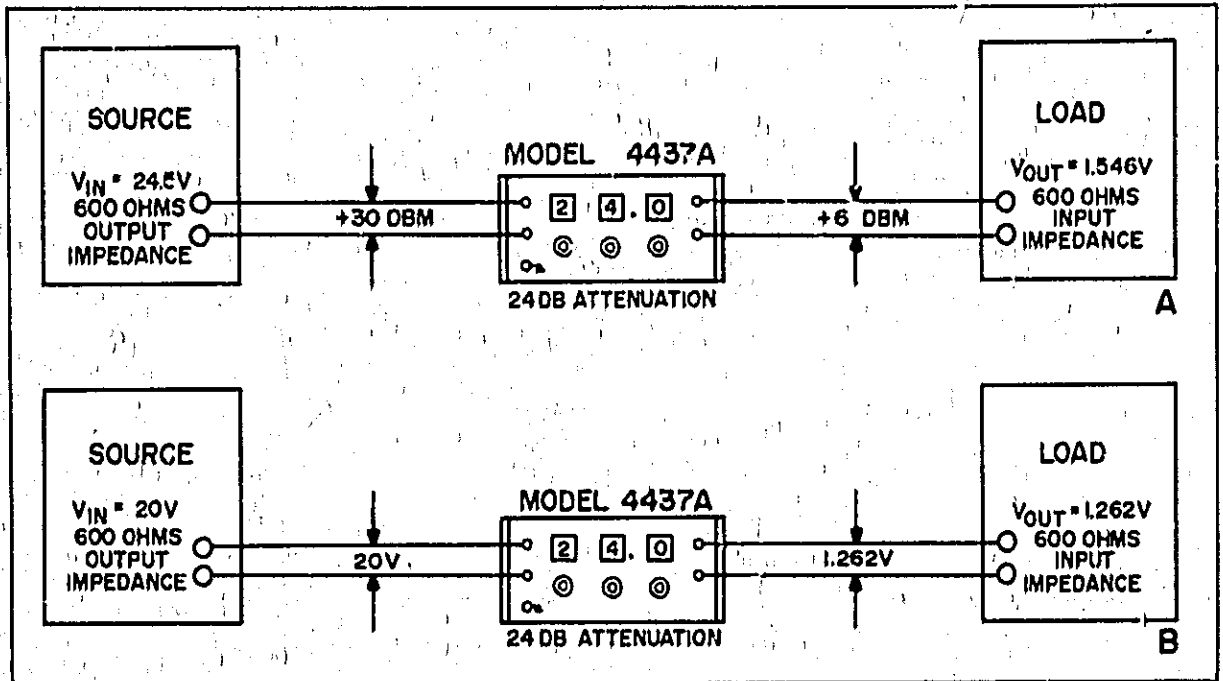
Figure 3-3. Impedance Matched Connection
