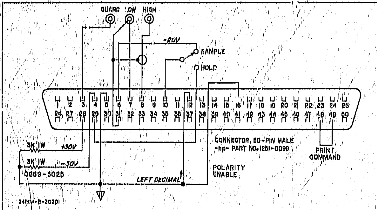
Figure 5-2. Suggested Test Fixture Schematic.
