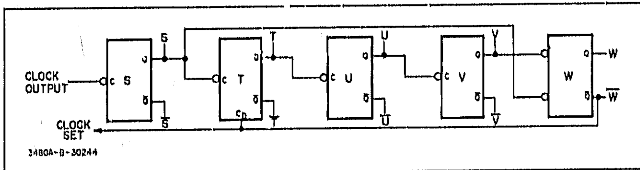
Figure 4-8. 18-Pulse Counter.
