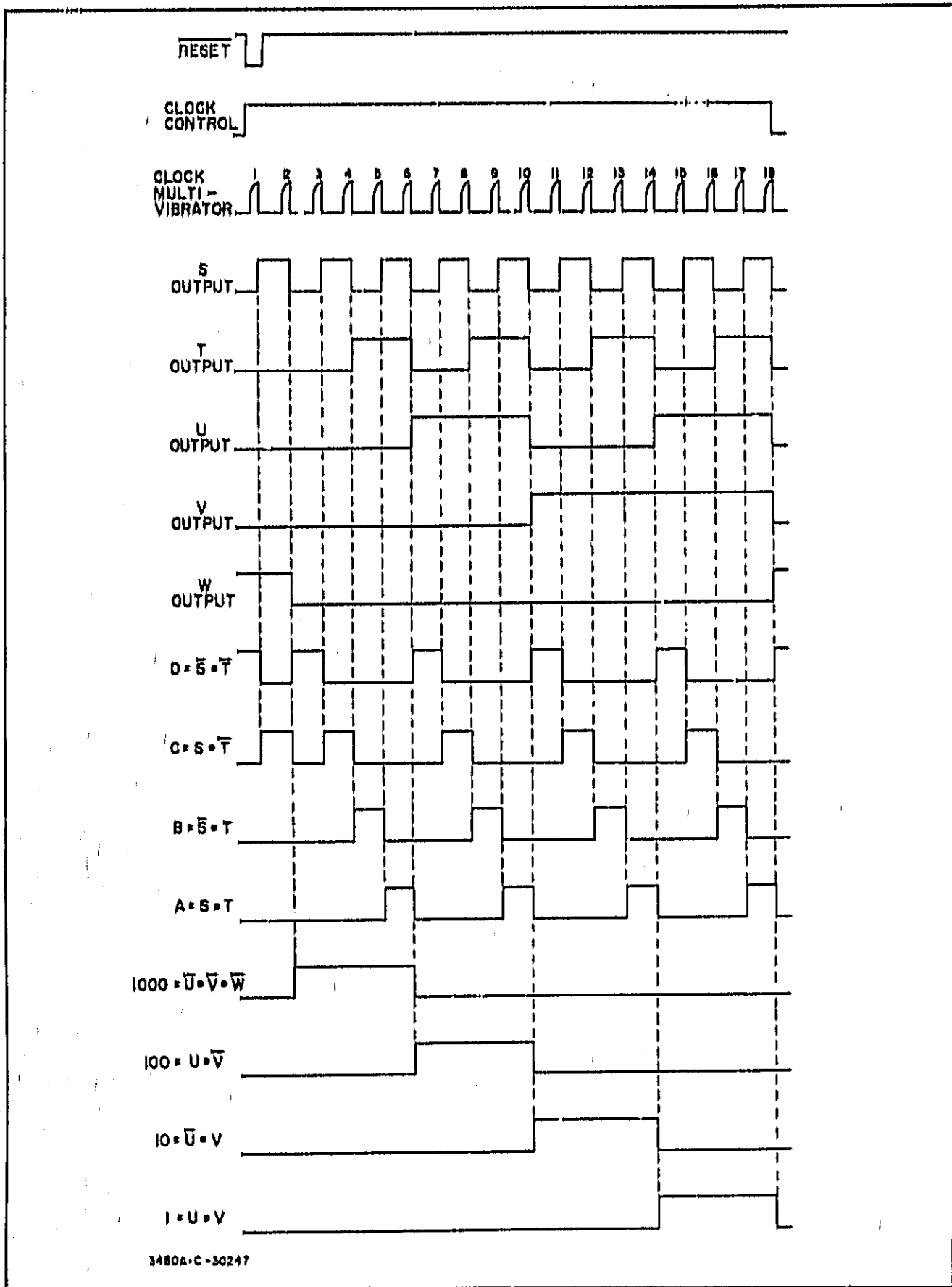
Figure 4-10. Clock and Counter Timing Sequence.
