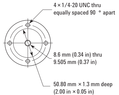
Flanged Shaft
