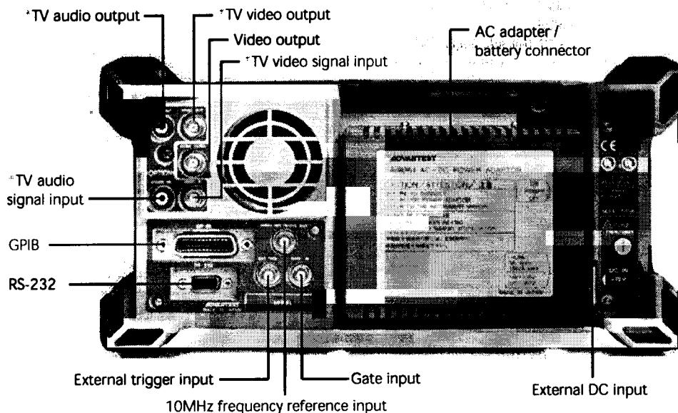
Rear panel
