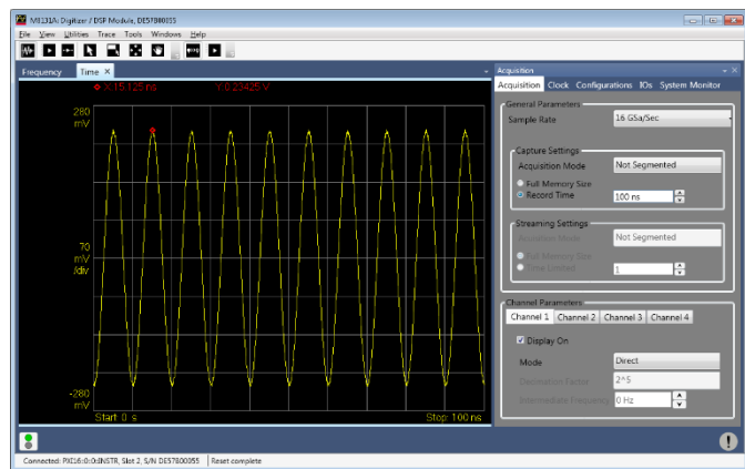
M8131A Soft Front Panel
