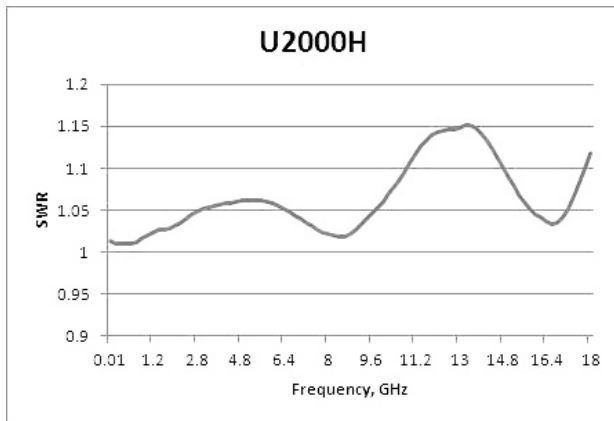
Typical SWR for U2000H sensor (25 °C ± 10 °C)
