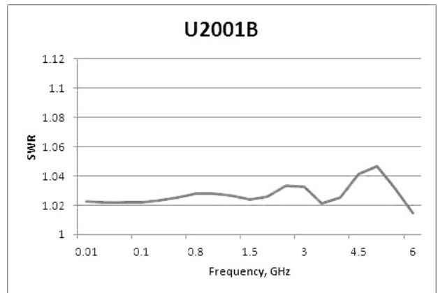
Typical SWR for U2001B sensor (25 °C ± 10 °C)
