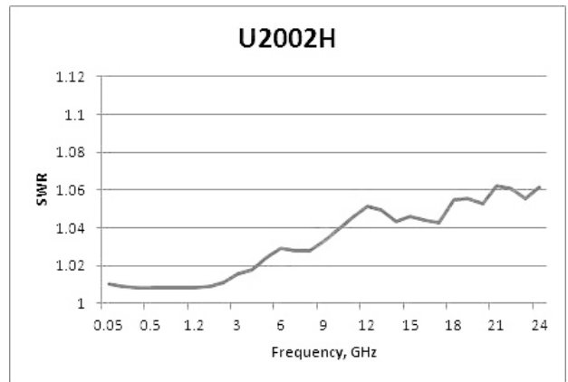
Typical SWR for U2002H sensor (25 °C ± 10 °C)
