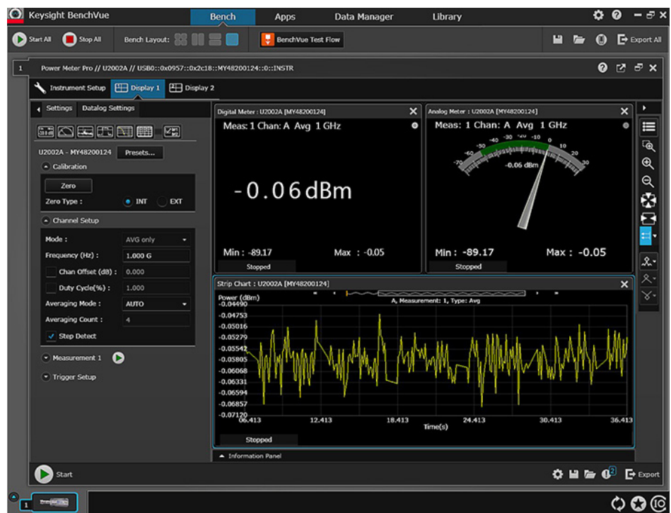
Digital meter, analog meter and datalog view.
