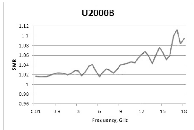
Typical SWR for U2000B sensor (25 °C ± 10 °C)
