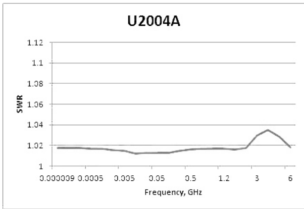
Typical SWR for U2004A sensor (25 °C ± 10 °C)
