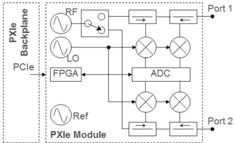
PXIe Vector Network Analyzer block diagram
