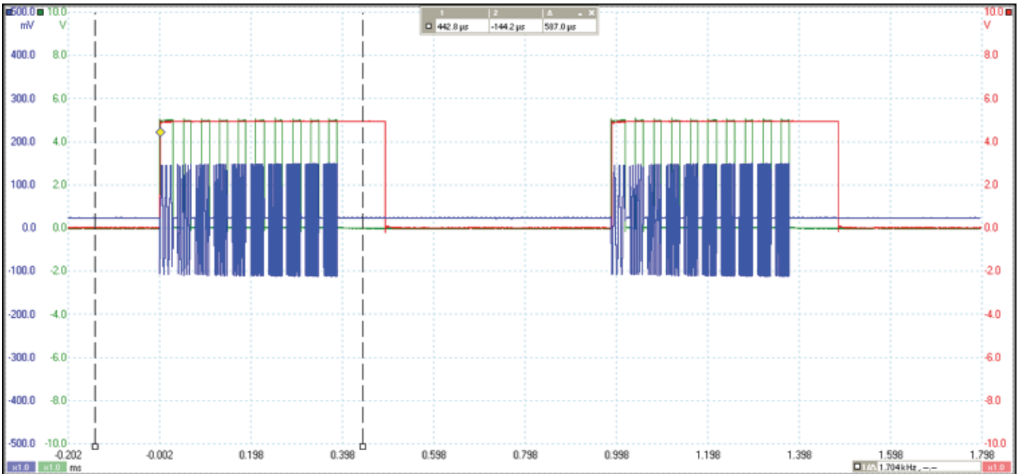
Figure 2: 10 point sweep with 50 \mu s step time.
