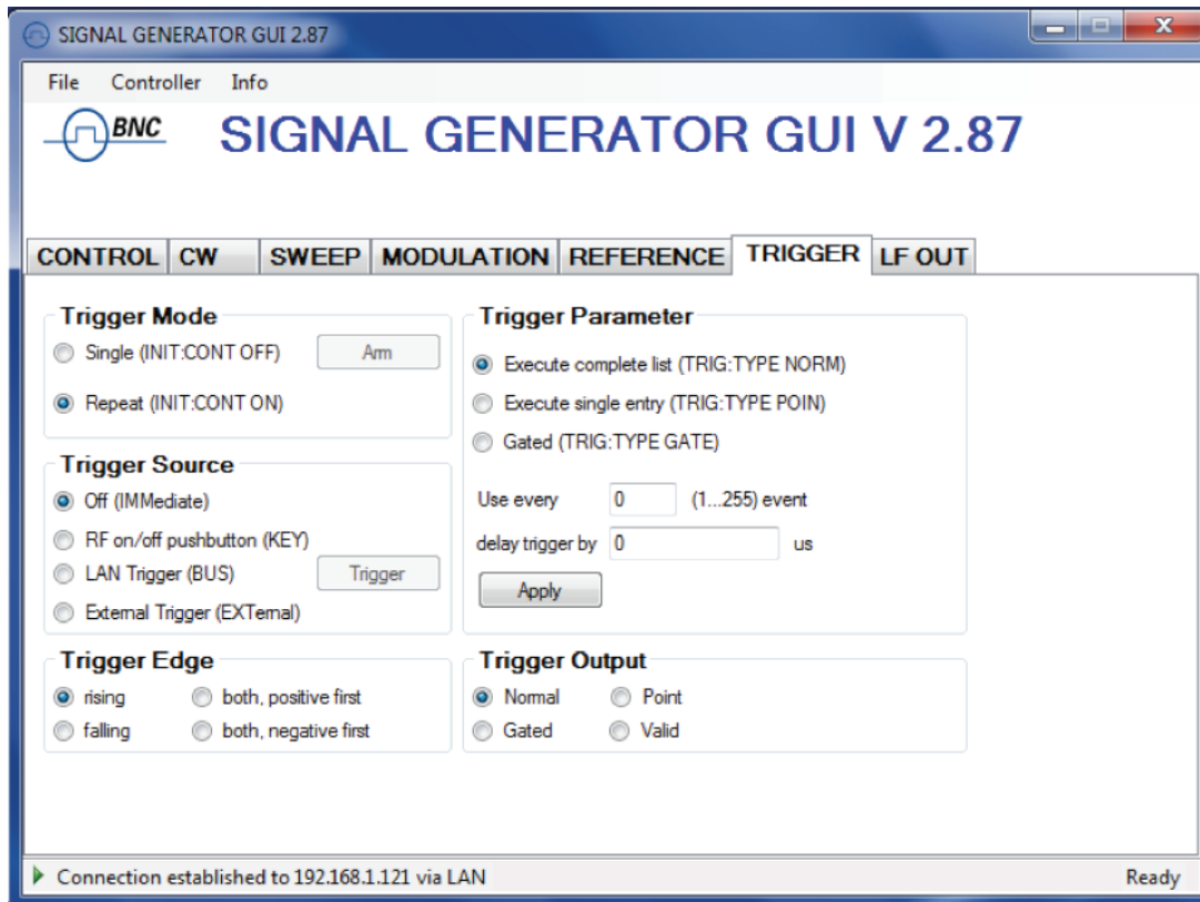
Figure 2: GUI trigger settings.
