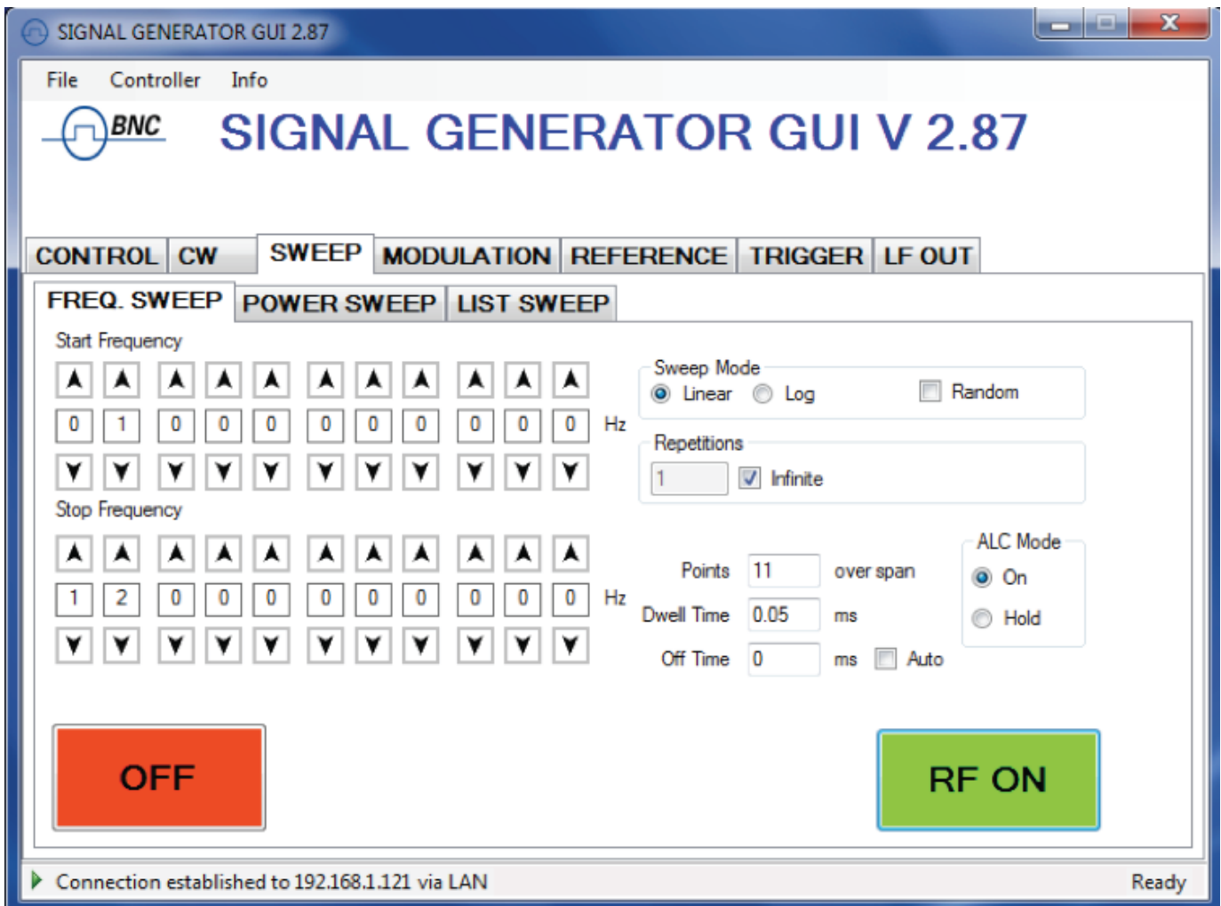
Figure 3: GUI sweep settings
