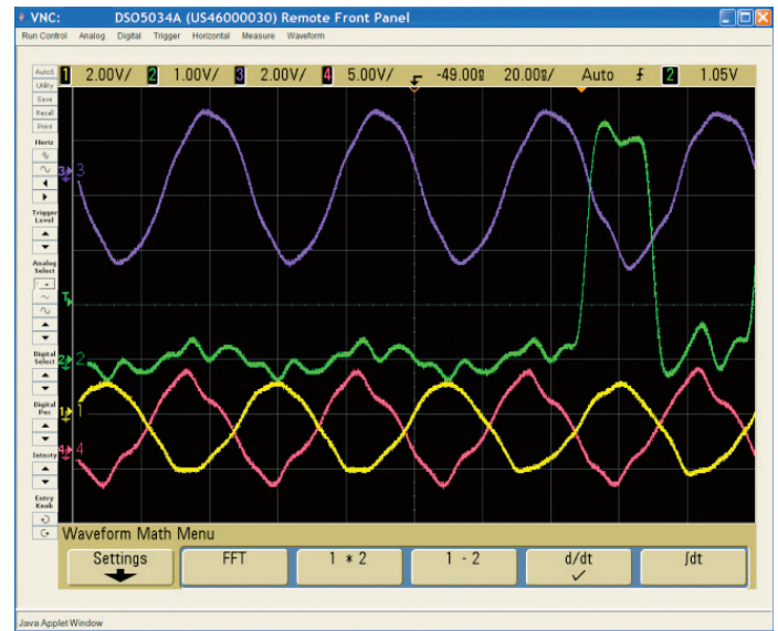
Keysight Remote Front Panel running in a web browser.
