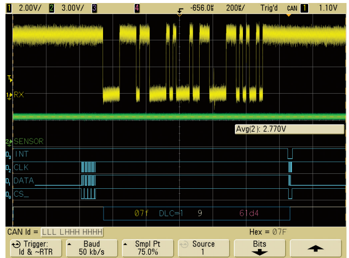
Random errors observed in CAN decode while triggering on data frame ID: 07FHEX.
